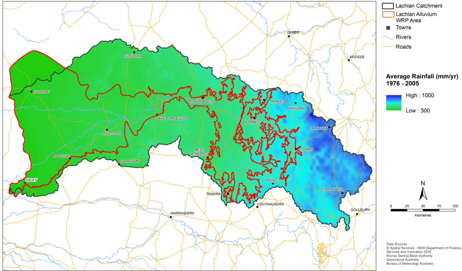
Figure 4 Average annual rainfall map of the Lachlan catchment (Bureau of Meteorology—BOM, 2008) 8
