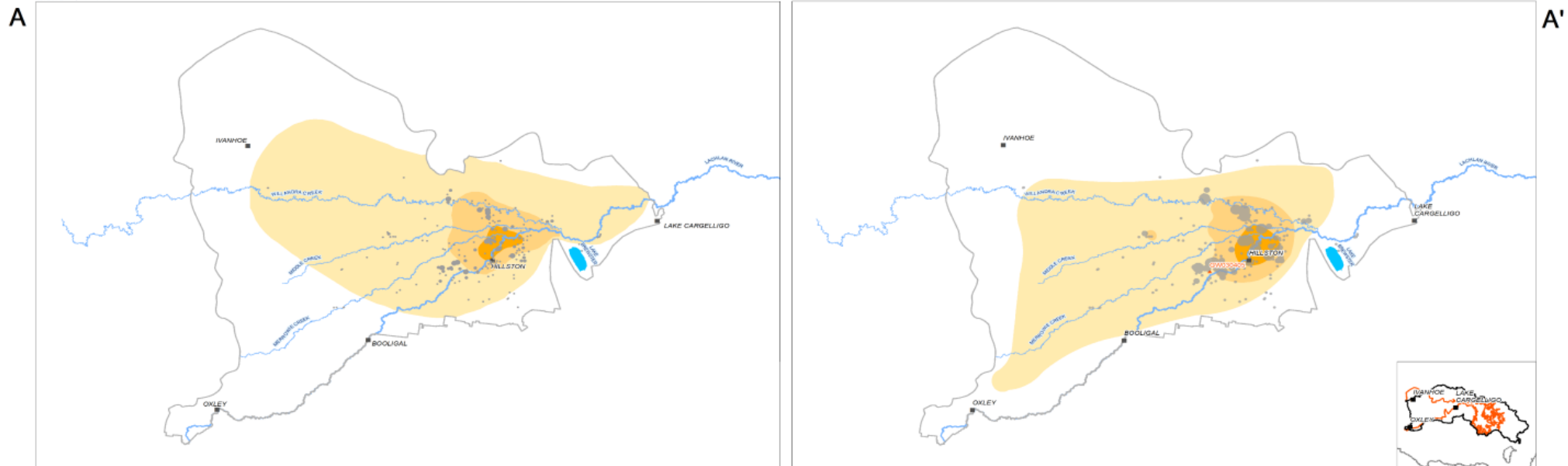
Change in Recovered Water Levels: 2005/2006 - 2015/2016 (Shallow Aquifer System)
