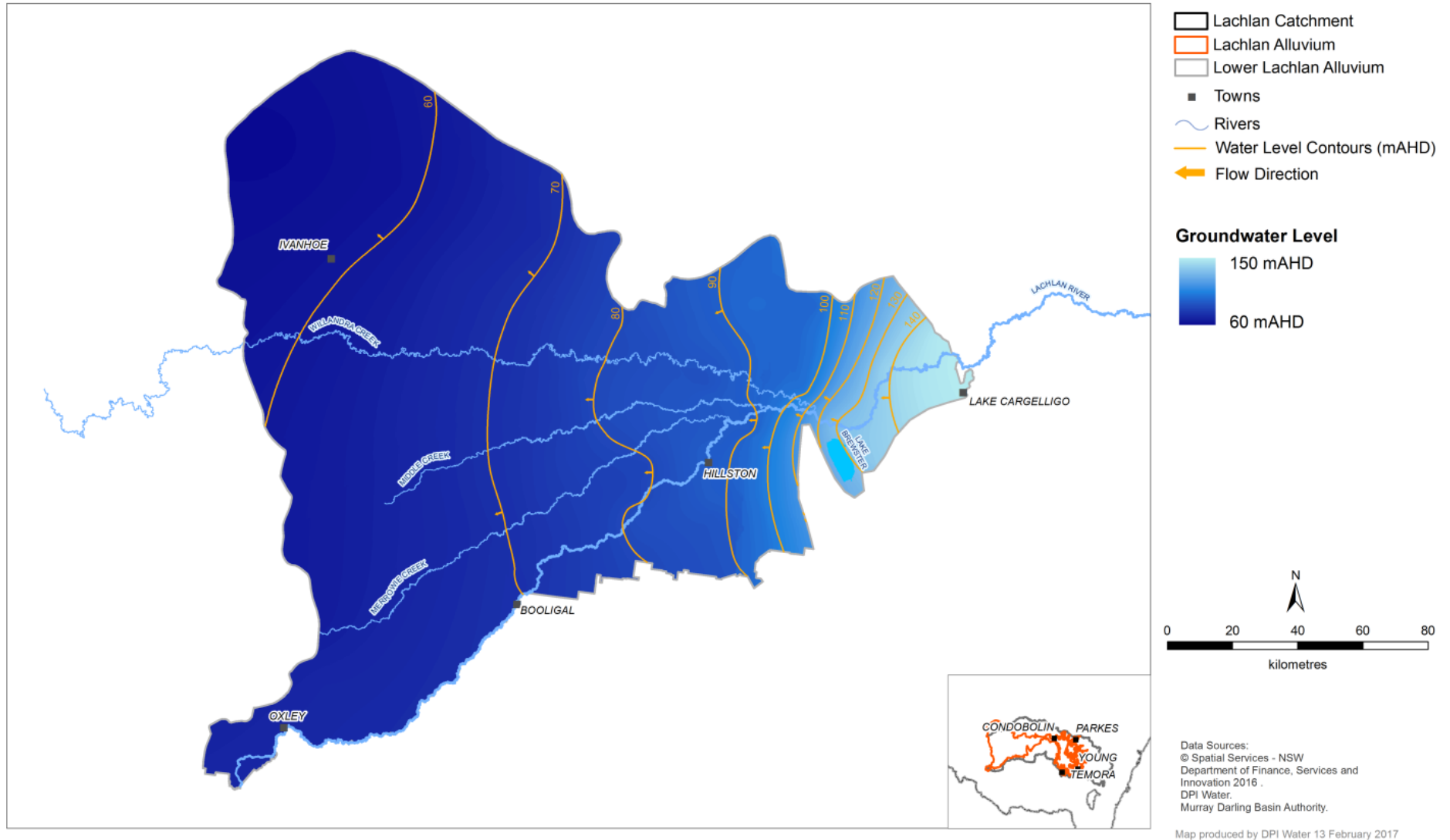
Figure 18 Location map Lower Lachlan Alluvium showing groundwater flow direction (deep aquifer)
