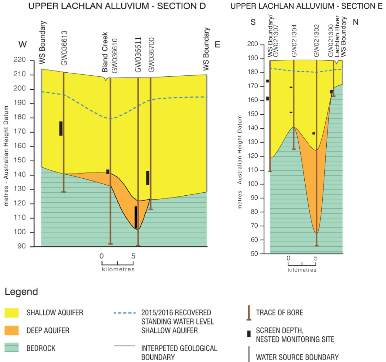
Figure 17 East-west section (Section D) and north-south section (Section E) through Upper Lachlan Alluvium
