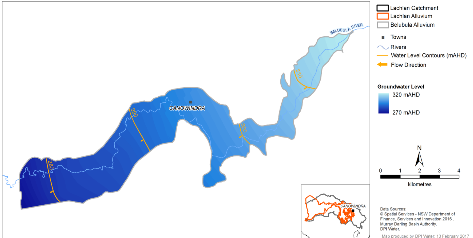
Figure 11 Location map of the Belubula Alluvium showing groundwater flow direction
