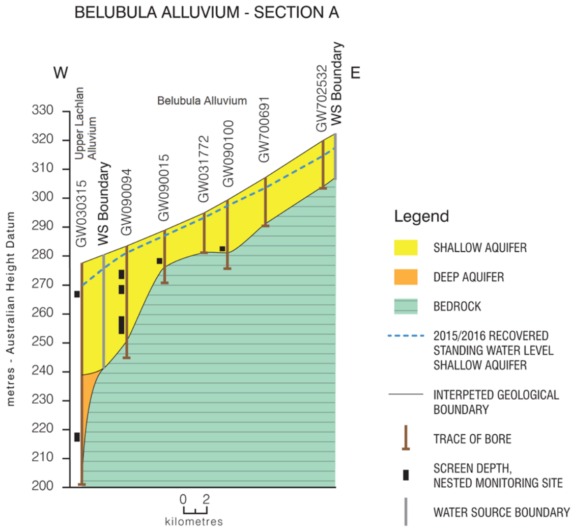
Figure 13 East-west long section through the Belubula Alluvium - Section A
