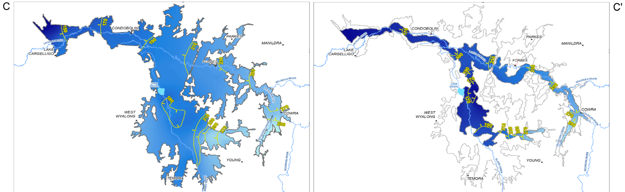
Deep System 2015/2016 Recovery
