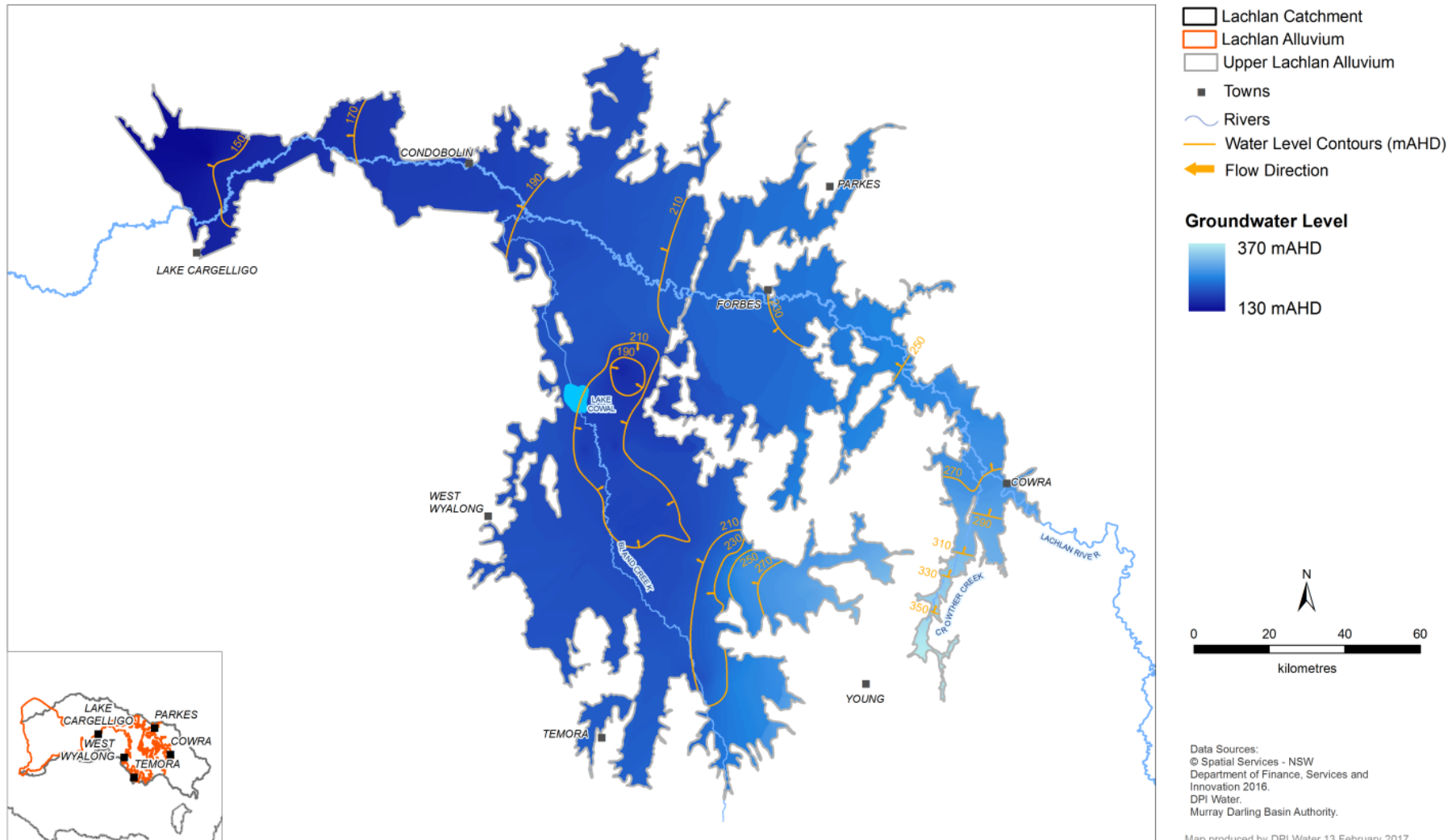
Figure 14 Location map of the Upper Lachlan Alluvium showing groundwater flow direction (deep aquifer)
