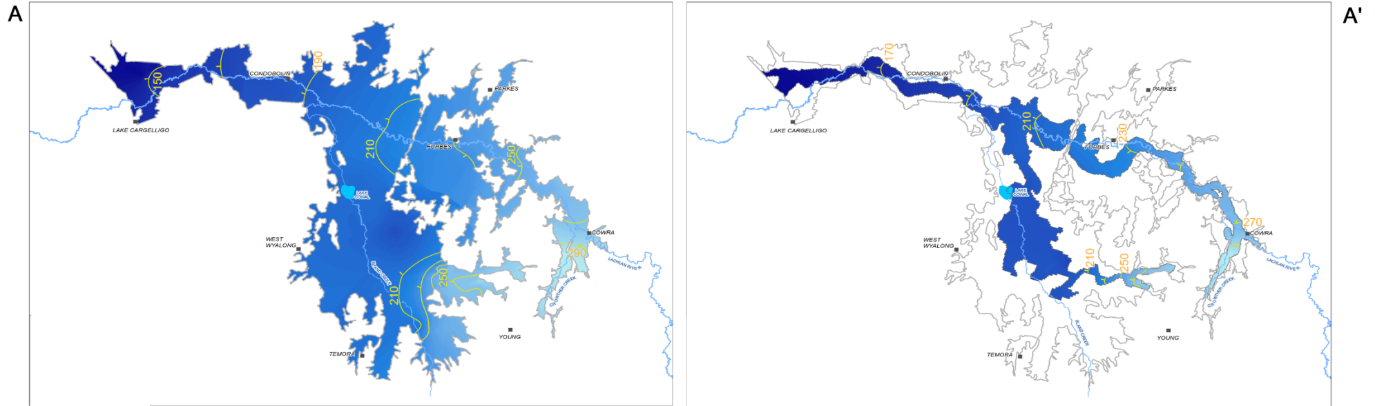
Shallow System Pre-development Recovery
