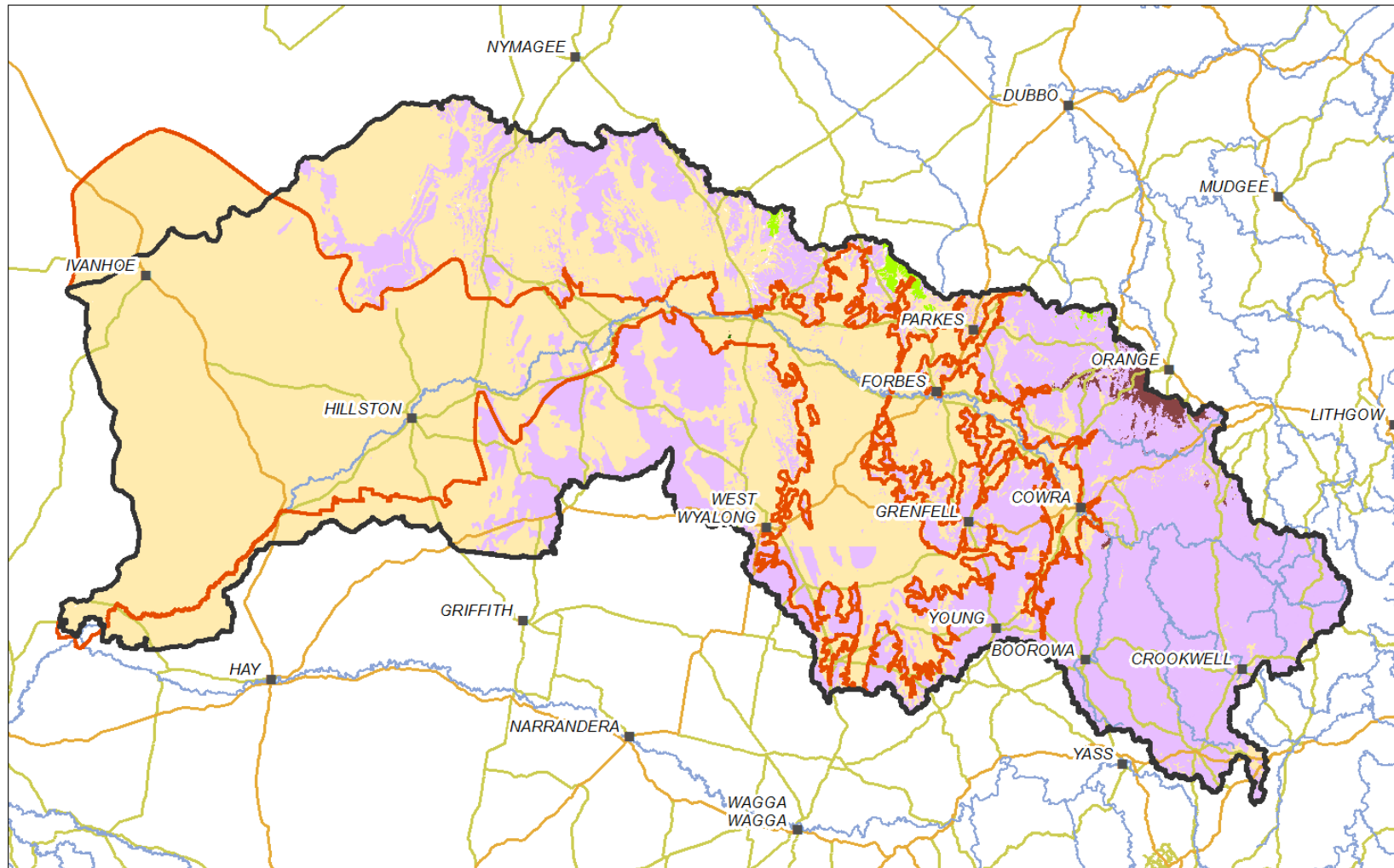
Figure 10 Geology of the Lachlan catchment
