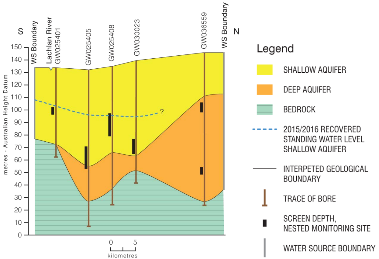
Figure 21 North-south section (Section G) through Lower Lachlan Alluvium
